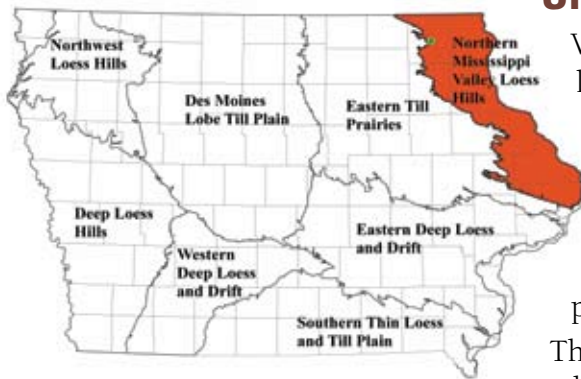
Figure 1. Northern Mississippi Valley Loess Hills and study site.
