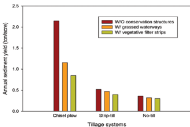
Figure 2. Impact of tillage systems and conservation structures on amount of soil leaving the field.
