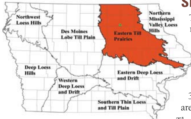
Figure 1. Eastern Till Prairie and study site.
